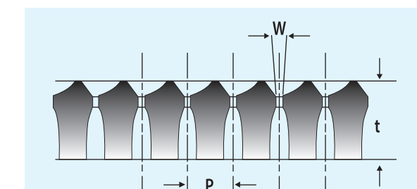
Grove and Slot Milled with Contoured Design.
